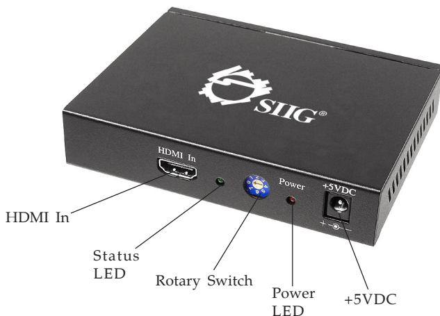
Figure 1: Front Panel
