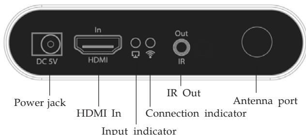
Figure 2: Transmitter (TX) - rear side
