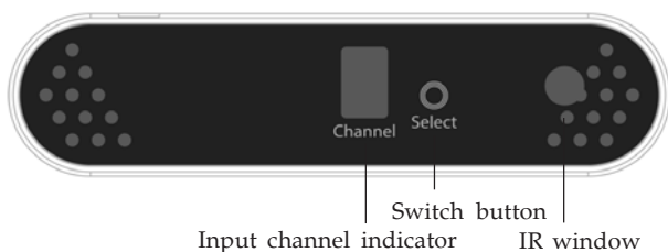
Figure 3: Receiver (RX) - front side
