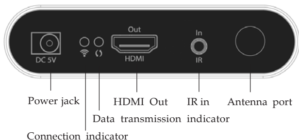
Figure 4: Receiver (RX) - rear side
