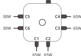
7 Ports Charging
