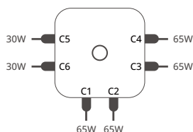
6 Ports Charging
