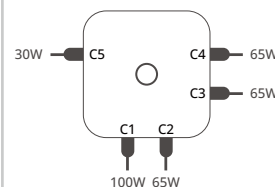
5 Ports Charging
