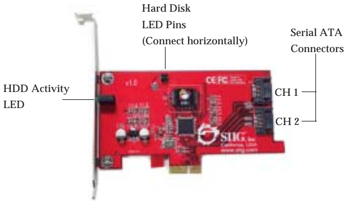
Figure 1. SATA II PCIe Board Layout
