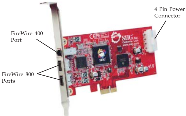
Figure 1: Board Layout
