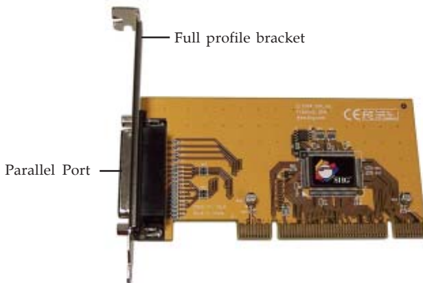
Figure 1. Layout
