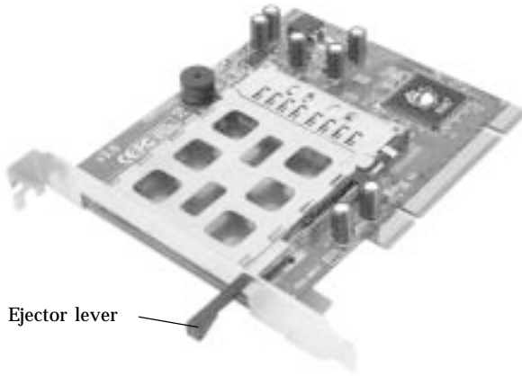
Figure 1. Layout
