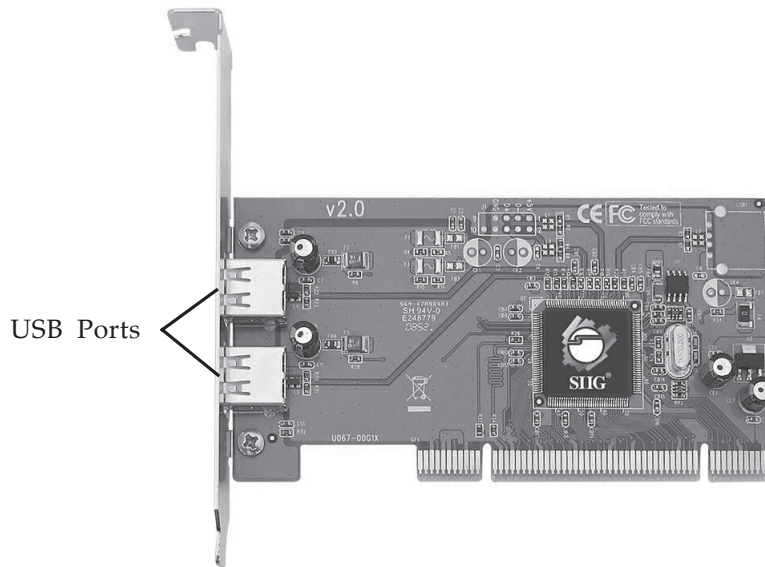
Figure 1. Layout
