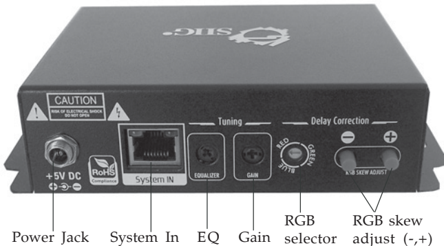
Figure 4: Rear view of Receiving (Rx) unit
