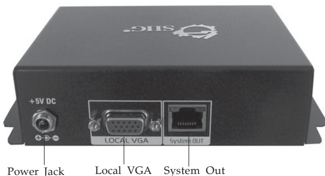
Figure 2: Rear view of Transmitting (Tx) unit
