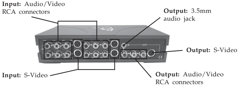
Figure 2: Rear Panel
