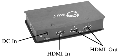
Figure 2: Rear Panel
