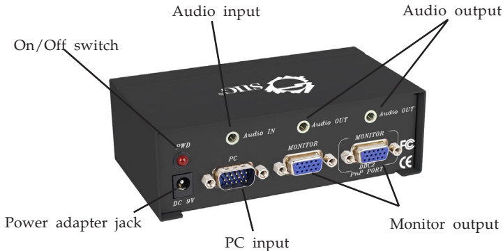
Figure 1. Rear Layout
