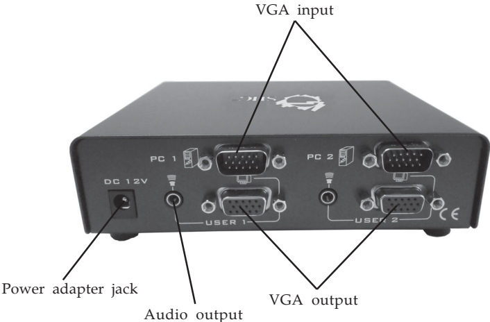
Figure 2: Rear Panel
