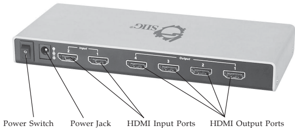
Figure 2: Rear Panel Layout
