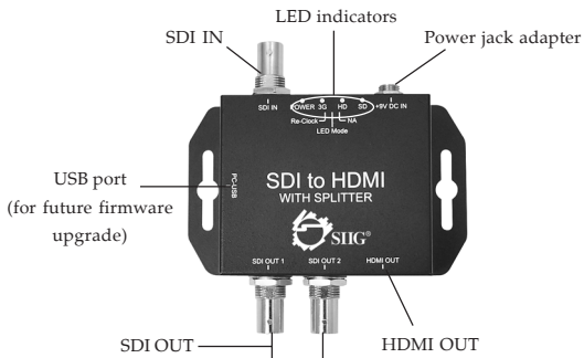
Figure 1: Layout
