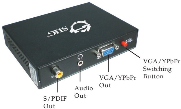
Figure 2: Rear Panel
