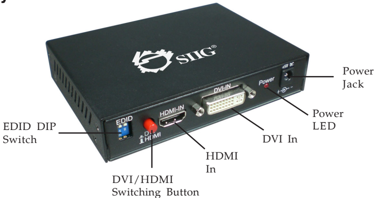
Figure 1: Front Panel
