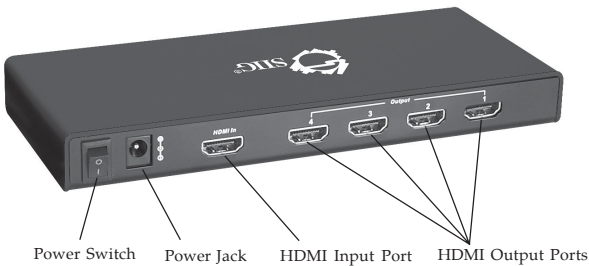
Figure 2: Rear Panel Layout
