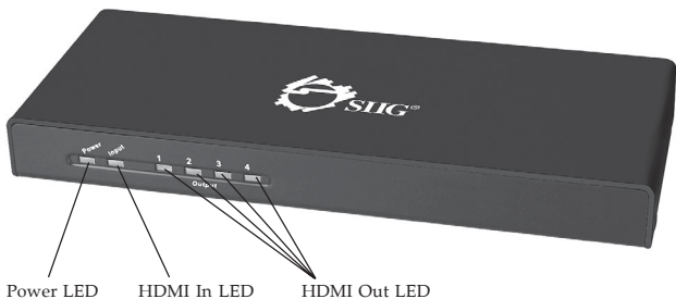
Figure 1: Front Panel Layout
