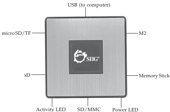
Figure 1: Layout
