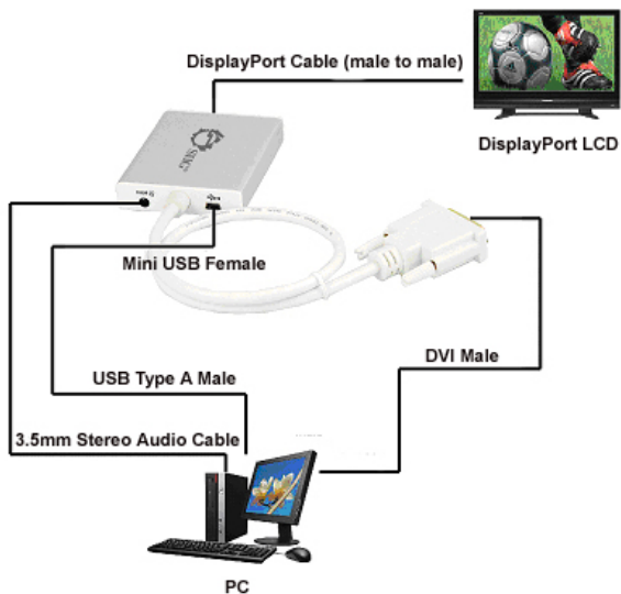
Figure 2: Application Diagram
