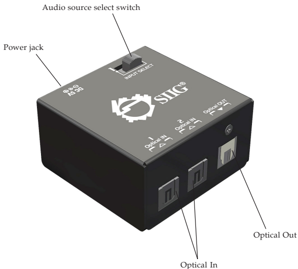
Figure 1: Layout
