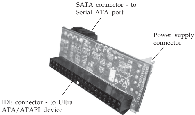
Figure 1: Layout
