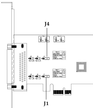
Figure 3: ID-P20211-S1 Pin Layout
