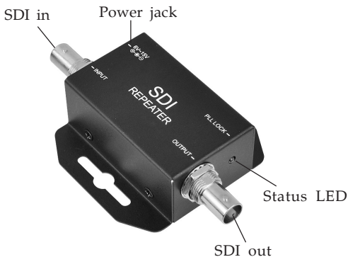
Figure 1: Layout
