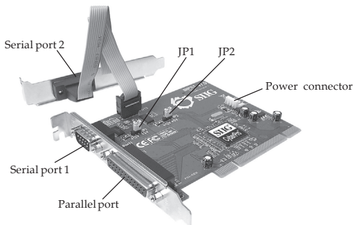
Figure 1: Board Layout
