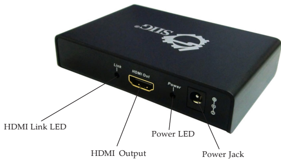
Figure 2: Back view
