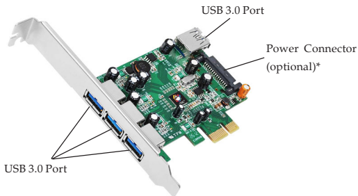
Figure 1: Board Layout
