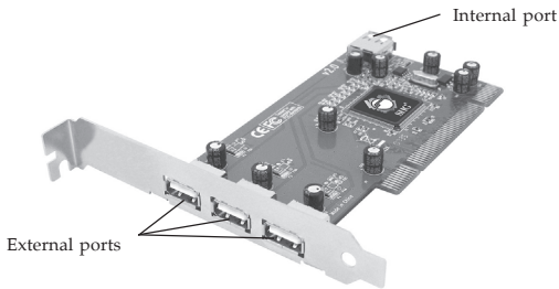
Figure 1: Board Layout
