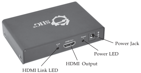
Figure 2: Back view
