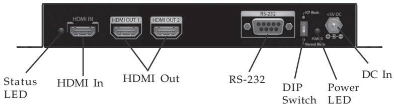
Figure 1: Rear Panel
