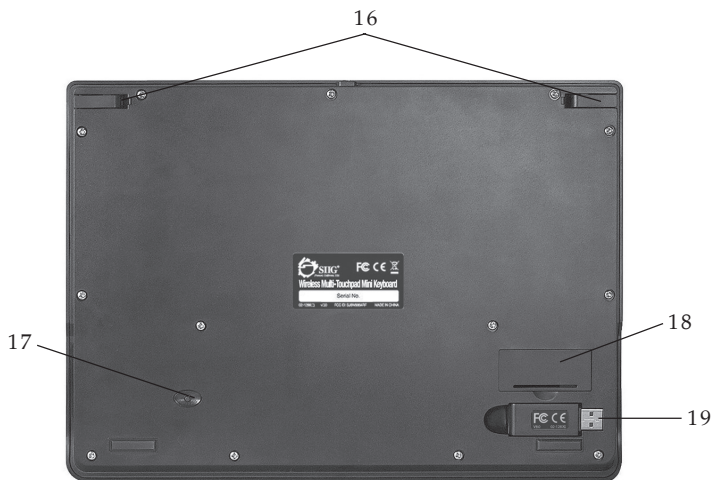
Figure 2: Bottom Layout
