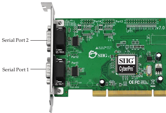
Figure 1: Board Layout
