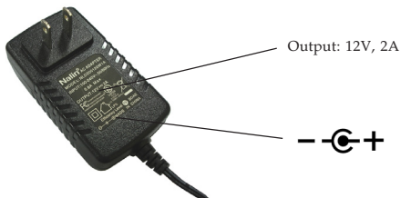
Figure 2: Power Adapter
