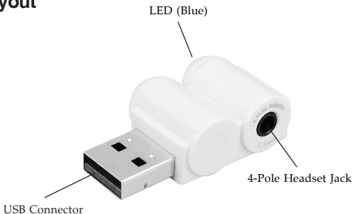
Figure 2: Layout
