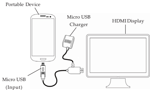
Figure 2: Device Connections
