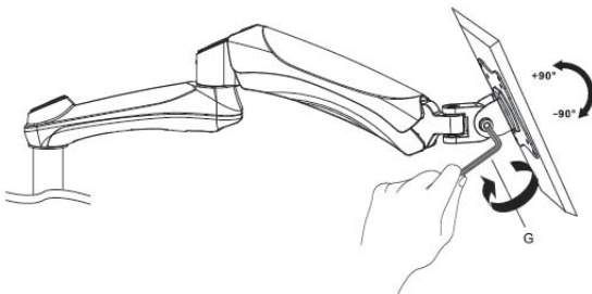
Adjust Tightness of Monitor Tilt and Swivel using 6mm Allen Key (G)
