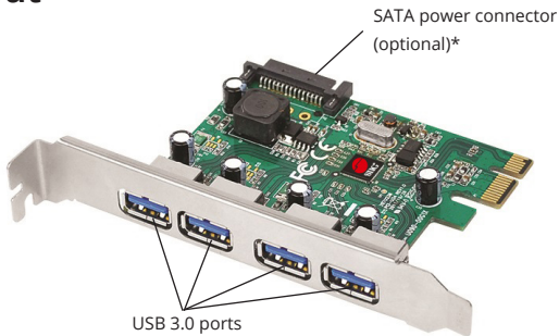
Figure 1: Layout
