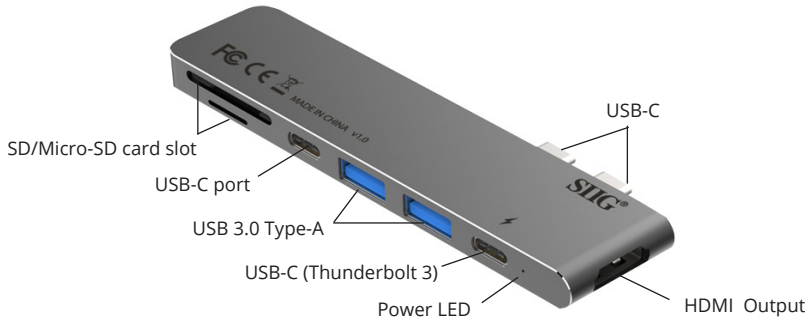
Figure 1: Thunderbolt 3 USB-C Hub HDMI with Card Reader & PD Adapter
