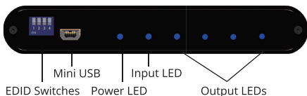
Figure 1: Front side
