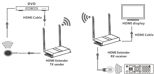
Point to point connection
