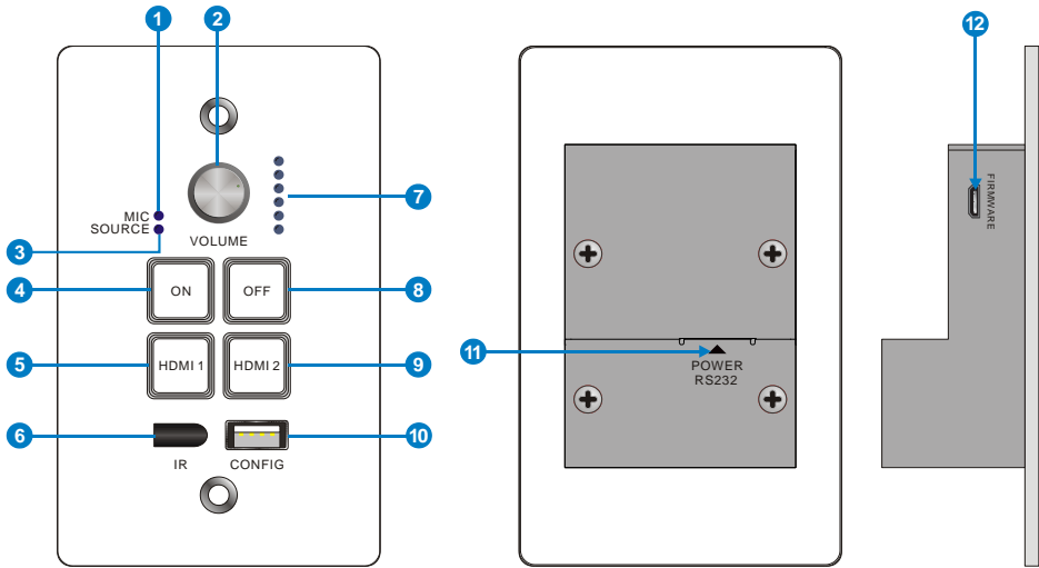
Figure 2-1 Control Panel
