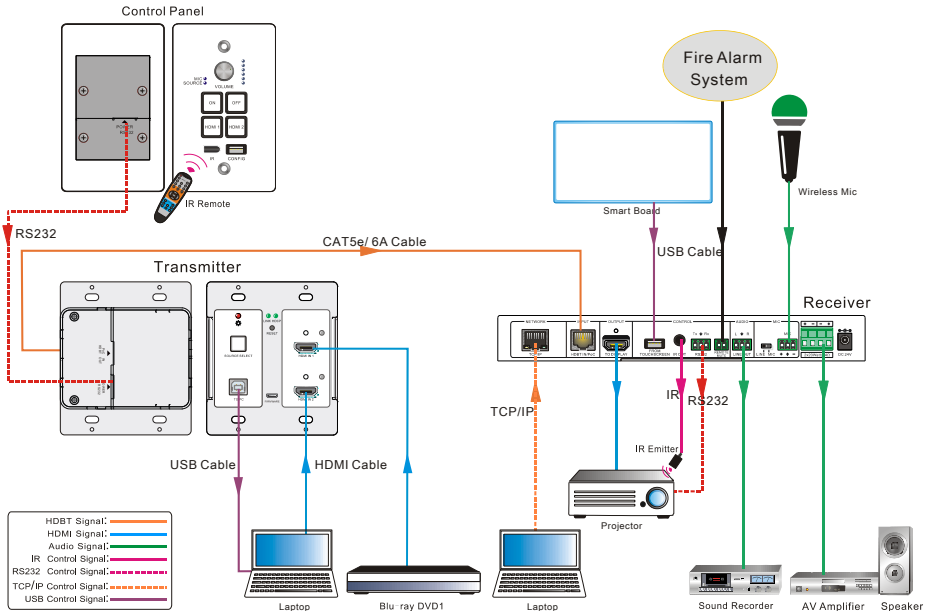
Figure 3-1 System Diagram
