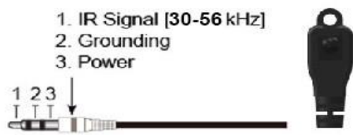
IR Receiver
