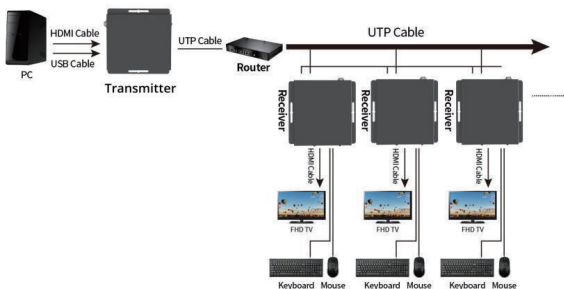
Figure 3: Application Diagram
